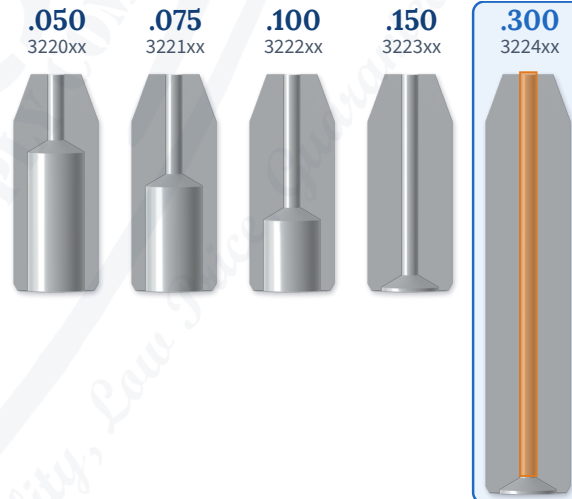
The five insert sections at one scale, this nozzle framed. Orange: the orifice bore, .300 in on this nozzle.
