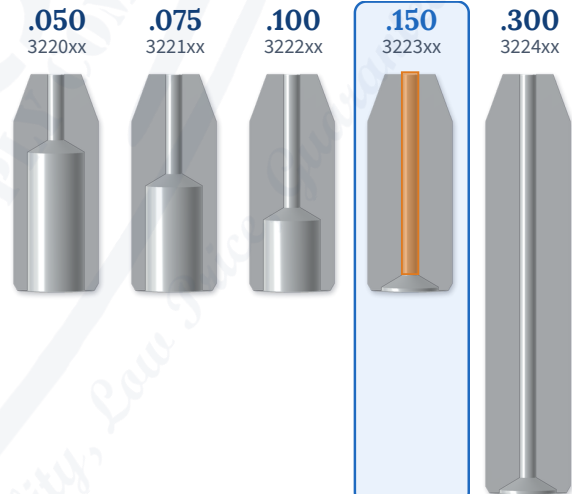
The five insert sections at one scale, this nozzle framed. Orange: the orifice bore, .150 in on this nozzle.
