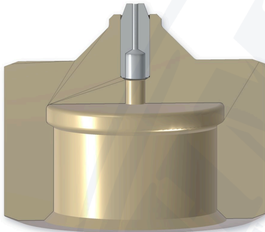
Cutaway, .100 in engagement: the stainless steel insert pressed into the phosphor brass body
