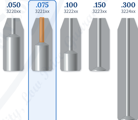
The five insert sections at one scale, this nozzle framed. Orange: the orifice bore, .075 in on this nozzle.
