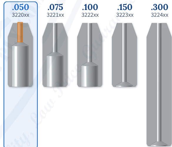
The five insert sections at one scale, this nozzle framed. Orange: the orifice bore, .050 in on this nozzle.
