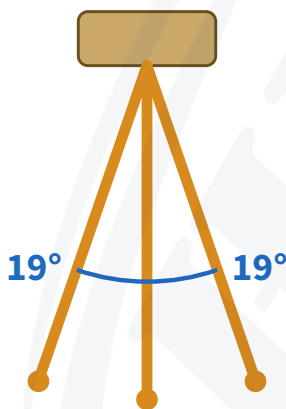
Triple 19°, front view schematic: 19 degrees between neighboring streams.
