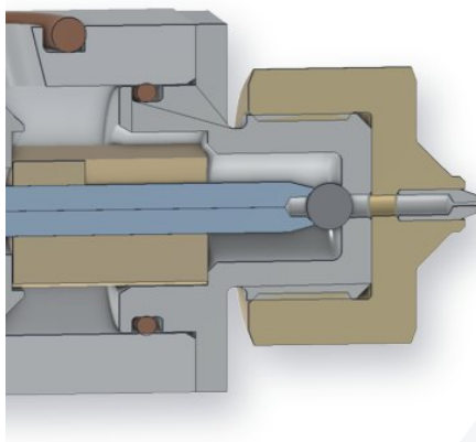
Mini ball and seat: brass nozzle (yellow), a ball on the needle closes against a seat (this module)
