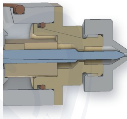
Mini NC: stainless steel nozzle (silver), the needle point seals at the orifice
