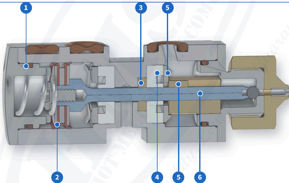
Cutaway of the mini ball and seat module, brass nozzle at the right end. Needle shown in blue. Numbers match the features below.
