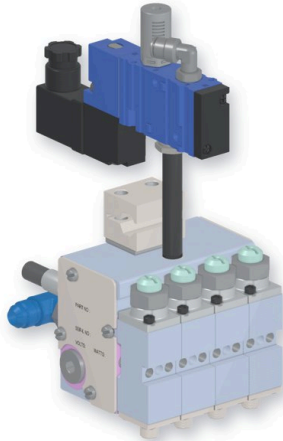
H204 Style 4 Module Gun, HMS-BC-430110123
