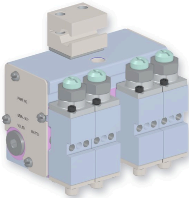
H204 Style 4 Module Gun, HMS-BC-410410000
